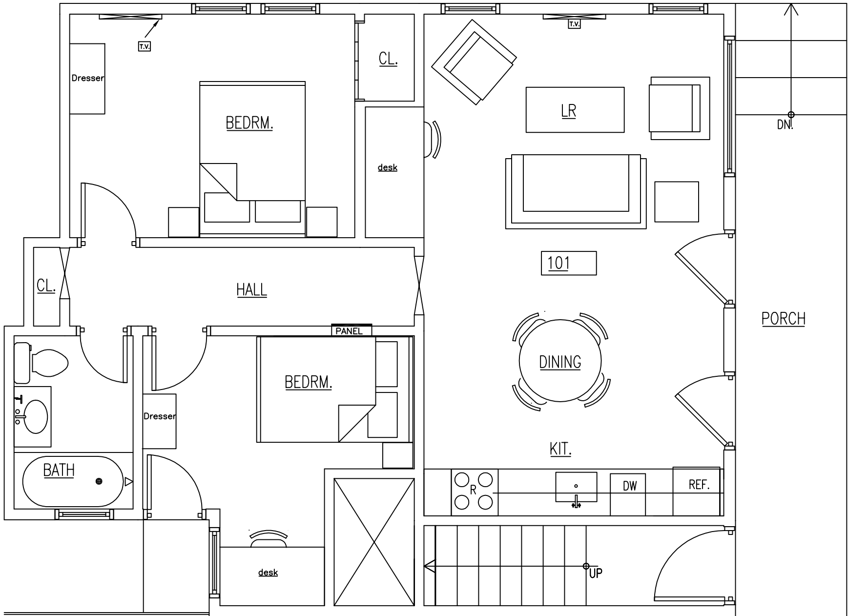
PROPOSED UNIT 101 PLAN
